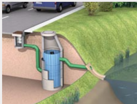
Run-off from highways
